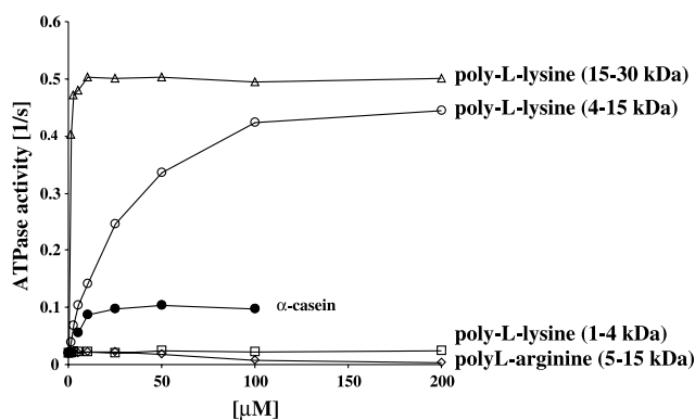
Fig. 1. Poly-L-lysine and \alpha -casein increase the ATPase activity of ClpB. Specific ATPase activities of ClpB (0.5 \mu M) were determined in the presence of increasing poly-L-lysine, poly-L-arginine and \alpha -casein concentrations.
